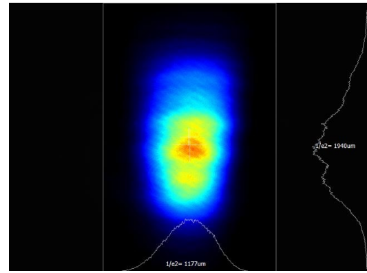
Typical far field (2.75 m from output aperture) beam profile. Non-circularized beam of a 0515 nm direct diode laser.
